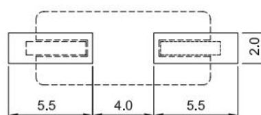
Top View Suggested Layout
